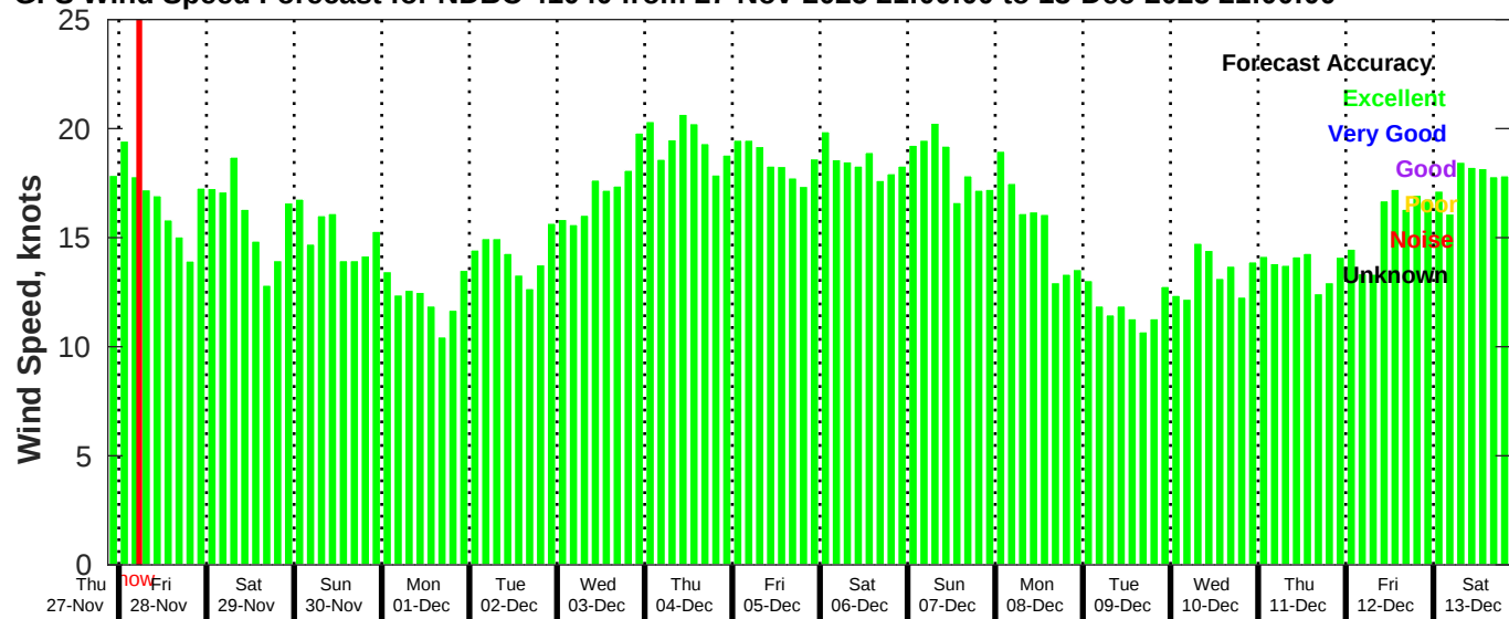
GFS Wind Speed Forecast for NDBC 41040 from 27-Nov-2025 21:00:00 to 13-Dec-2025 21:00:00
