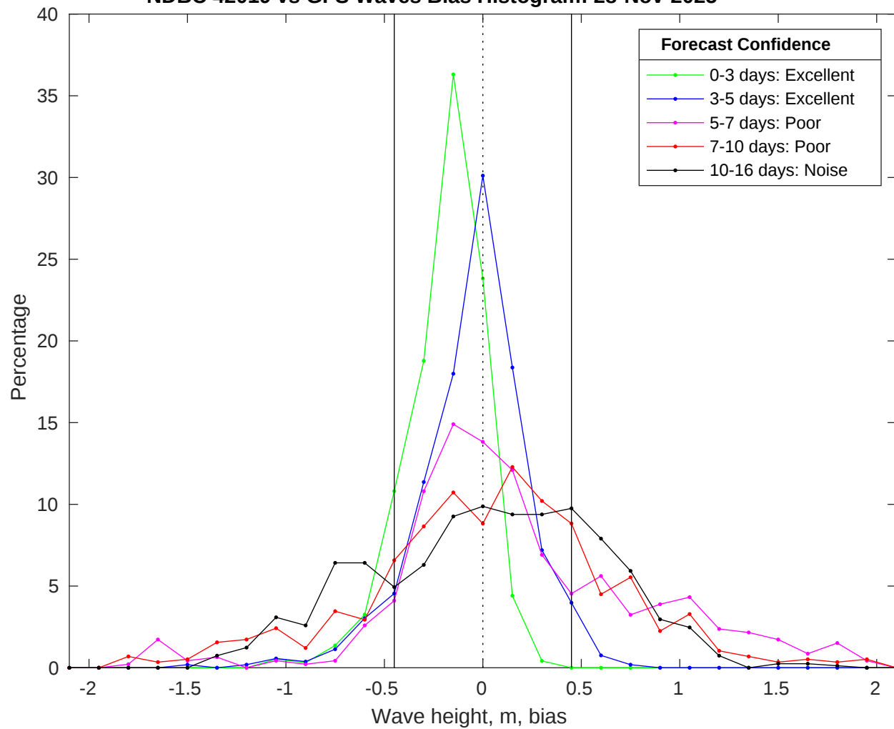
NDBC 42019 vs GFS Waves Bias Histogram: 28-Nov-2025
