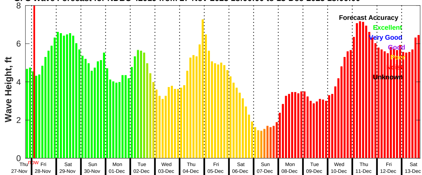
GFS Wave Forecast for NDBC 42019 from 27-Nov-2025 18:00:00 to 13-Dec-2025 18:00:00
