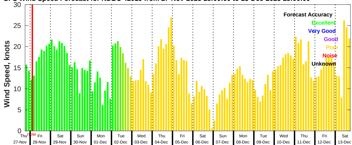
GFS Wind Speed Forecast for NDBC 42019 from 27-Nov-2025 18:00:00 to 13-Dec-2025 18:00:00
