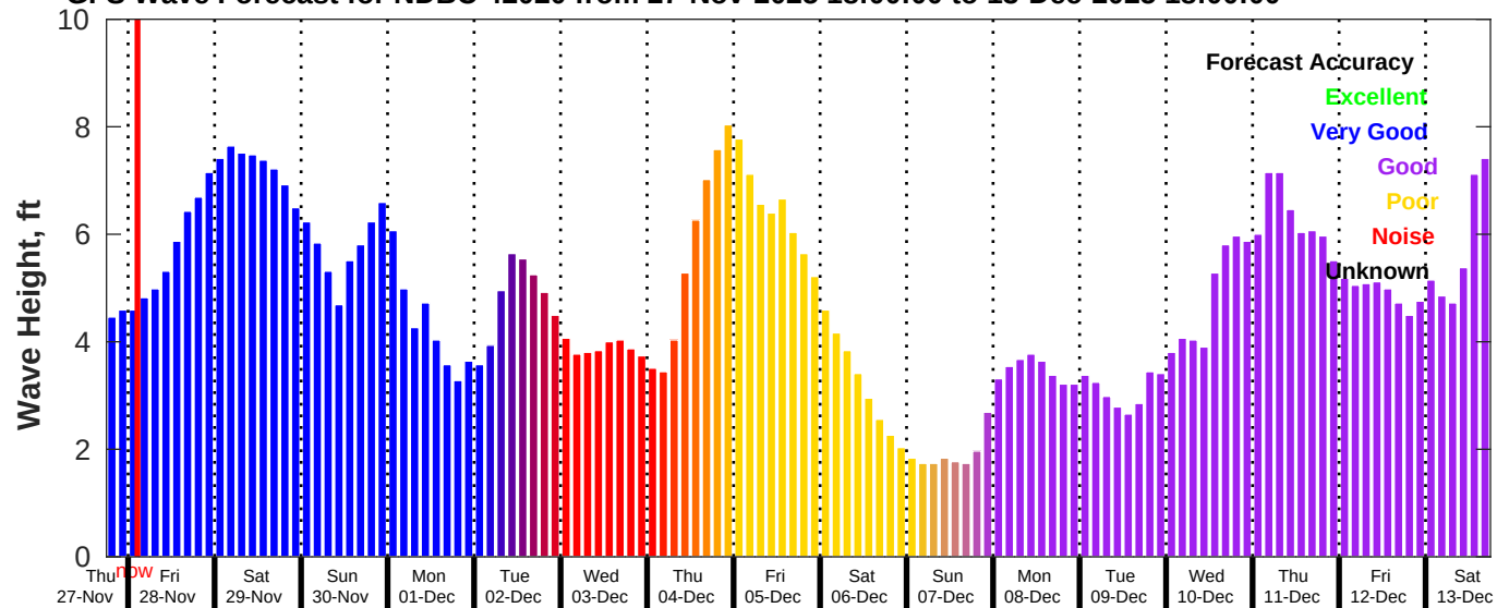
GFS Wave Forecast for NDBC 42020 from 27-Nov-2025 18:00:00 to 13-Dec-2025 18:00:00
