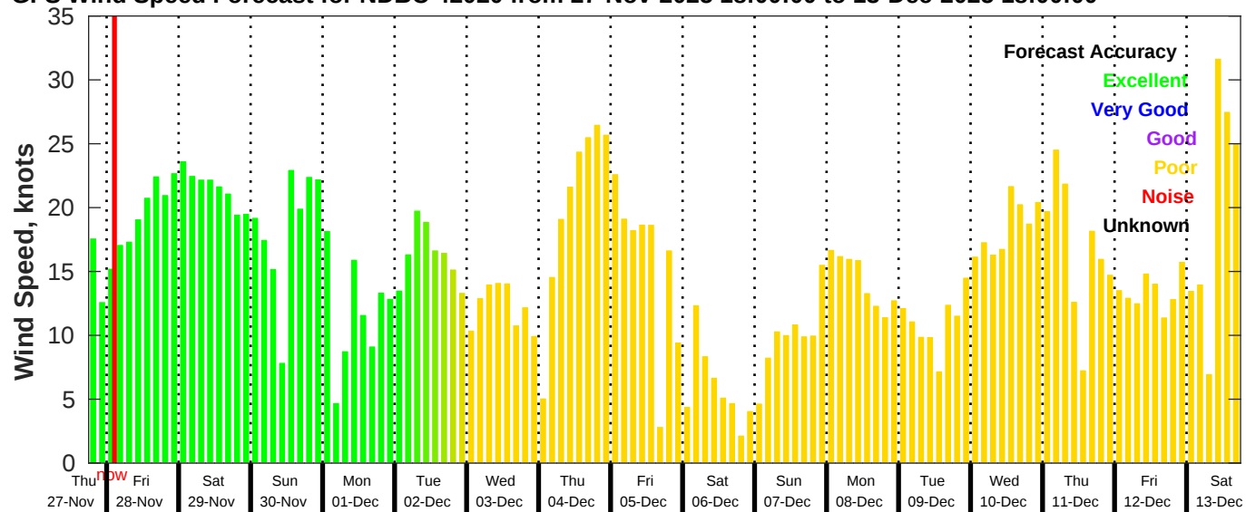
GFS Wind Speed Forecast for NDBC 42020 from 27-Nov-2025 18:00:00 to 13-Dec-2025 18:00:00
