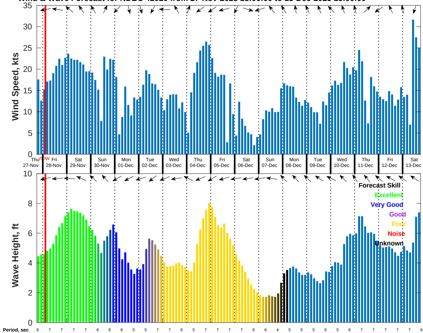
Wind & Wave Forecast for NDBC 42020 from 27-Nov-2025 18:00:00 to 13-Dec-2025 18:00:00
