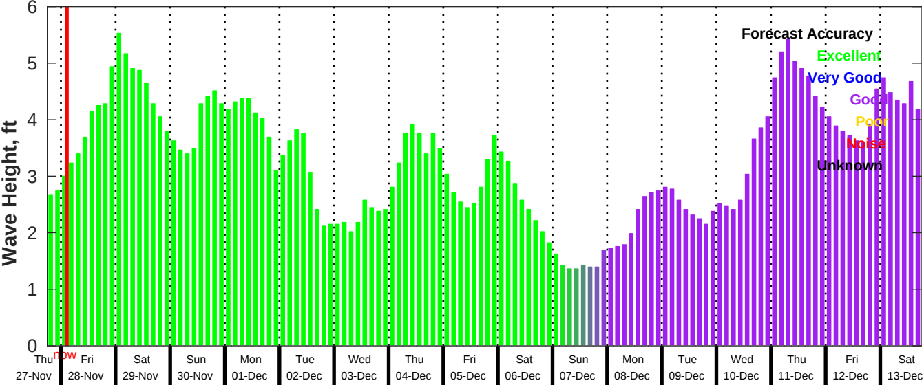
GFS Wave Forecast for NDBC 42035 from 27-Nov-2025 18:00:00 to 13-Dec-2025 18:00:00
