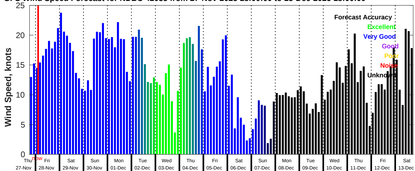
GFS Wind Speed Forecast for NDBC 42035 from 27-Nov-2025 18:00:00 to 13-Dec-2025 18:00:00
