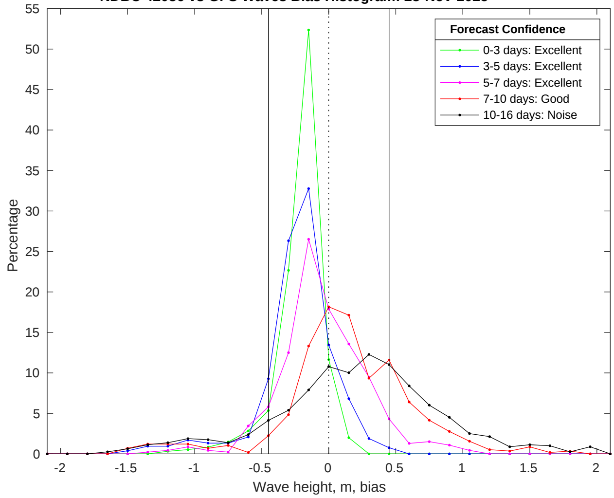
NDBC 42036 vs GFS Waves Bias Histogram: 28-Nov-2025
