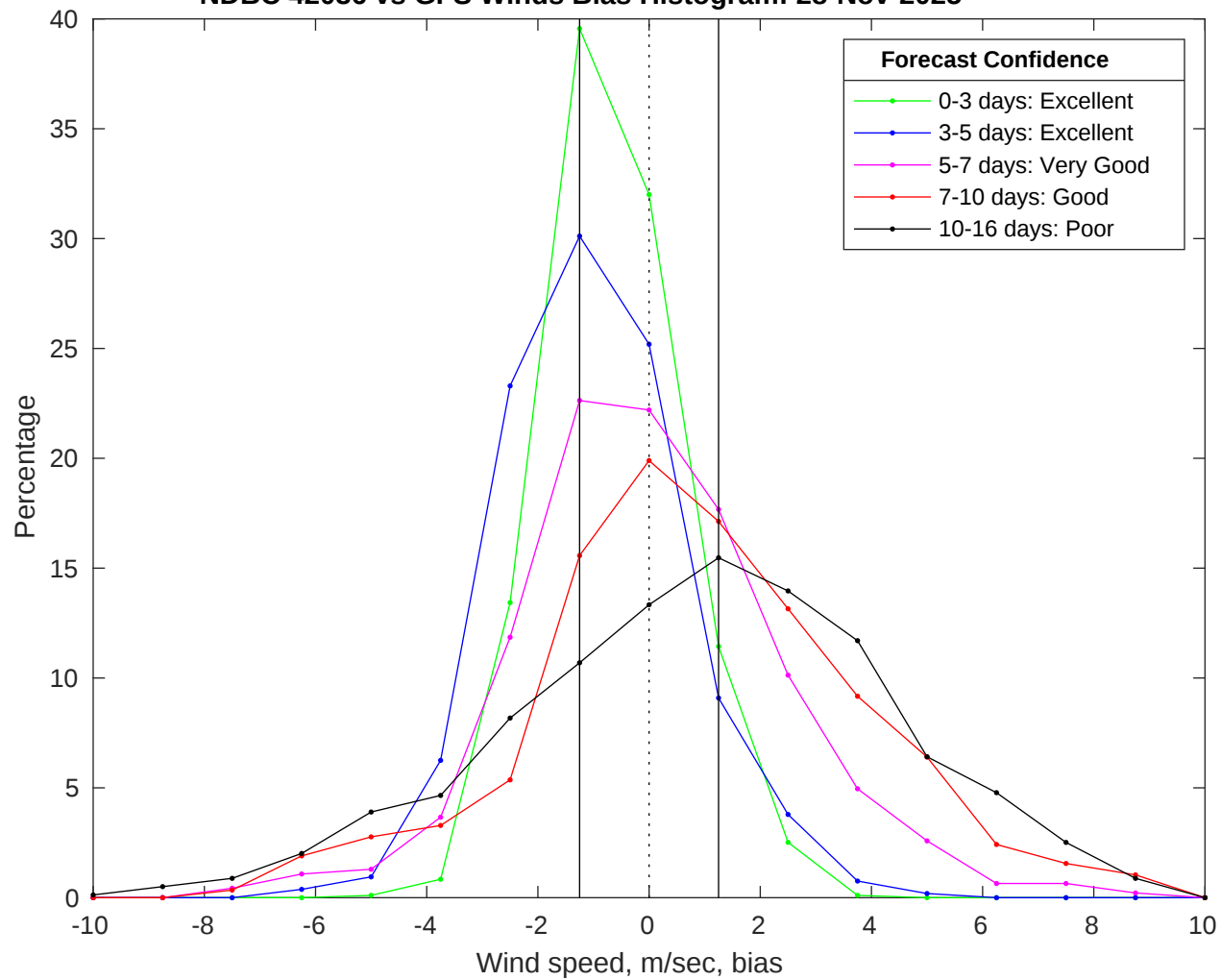
NDBC 42036 vs GFS Winds Bias Histogram: 28-Nov-2025
