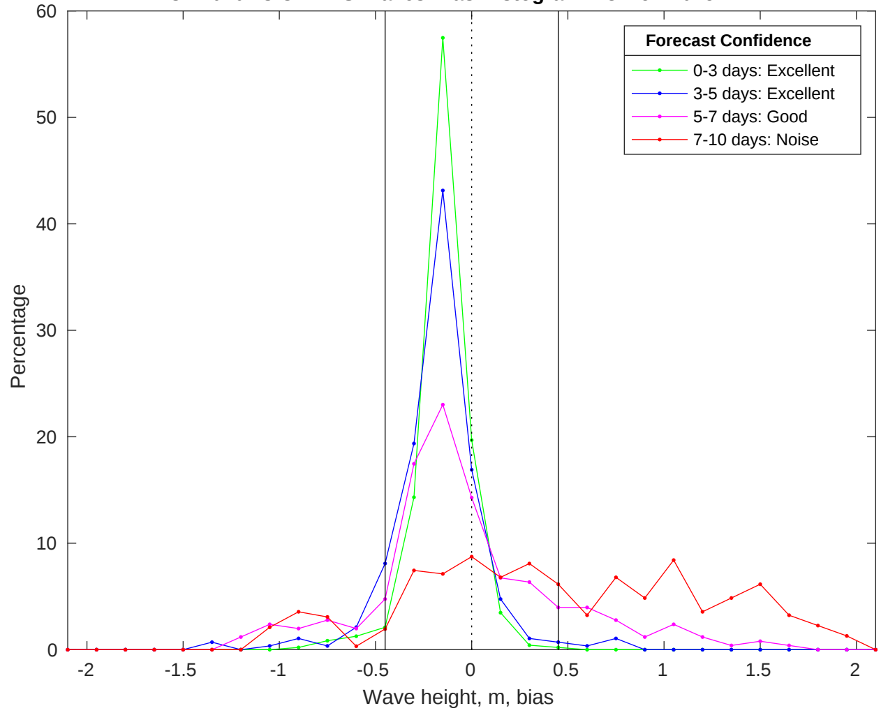
NDBC 42040 vs CMEMS Waves Bias Histogram: 28-Nov-2025
