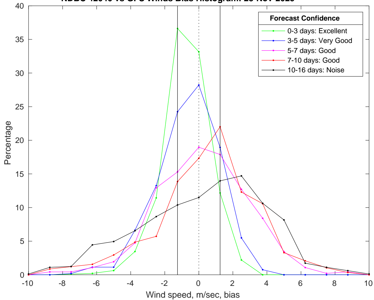
NDBC 42040 vs GFS Winds Bias Histogram: 28-Nov-2025
