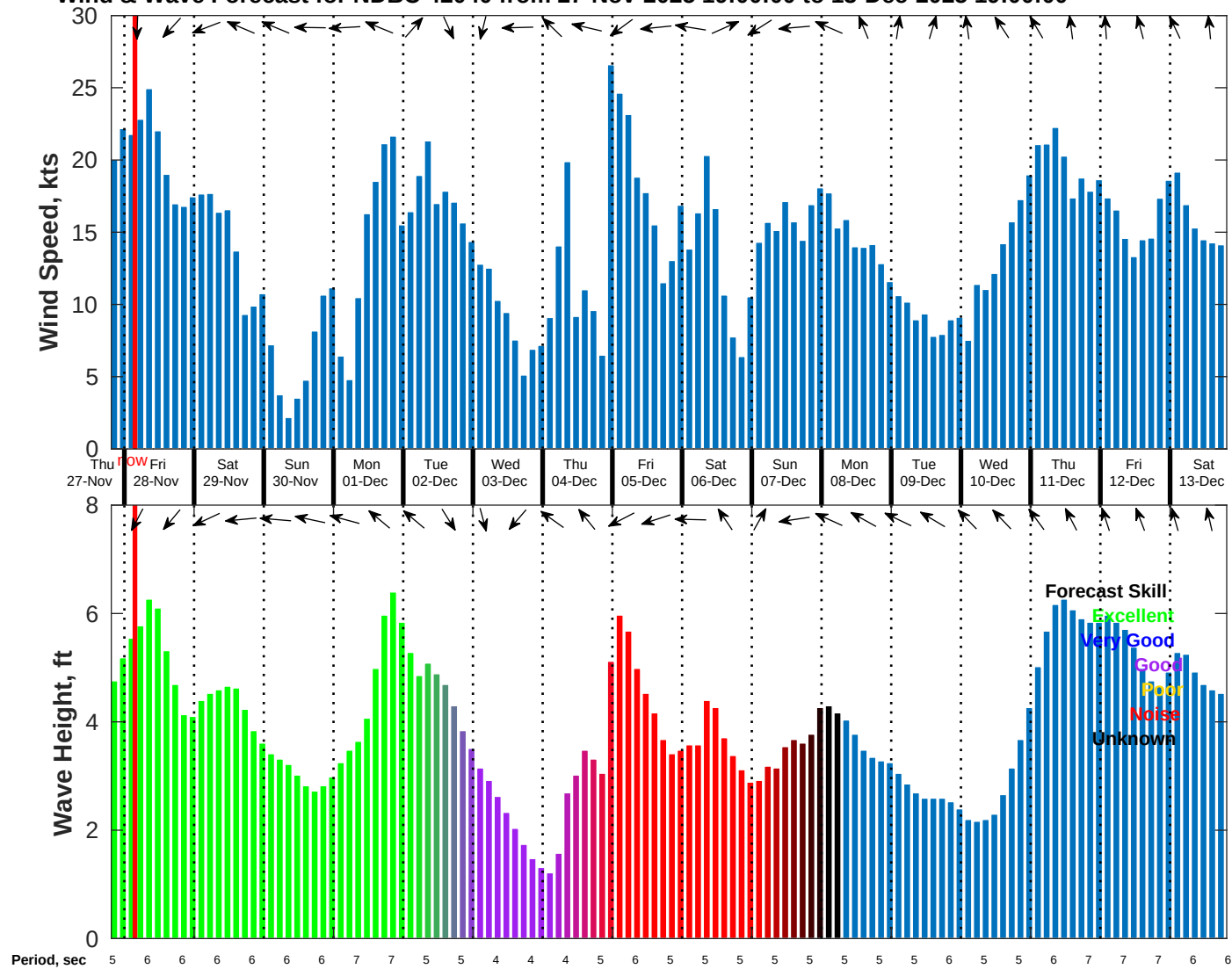
Wind & Wave Forecast for NDBC 42040 from 27-Nov-2025 19:00:00 to 13-Dec-2025 19:00:00
