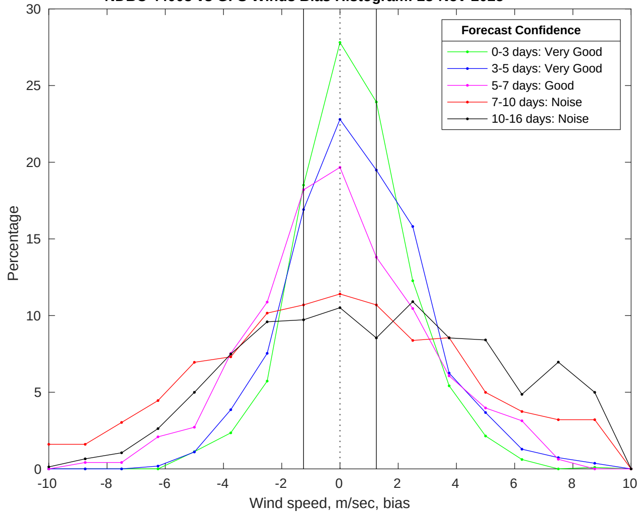
NDBC 44008 vs GFS Winds Bias Histogram: 28-Nov-2025
