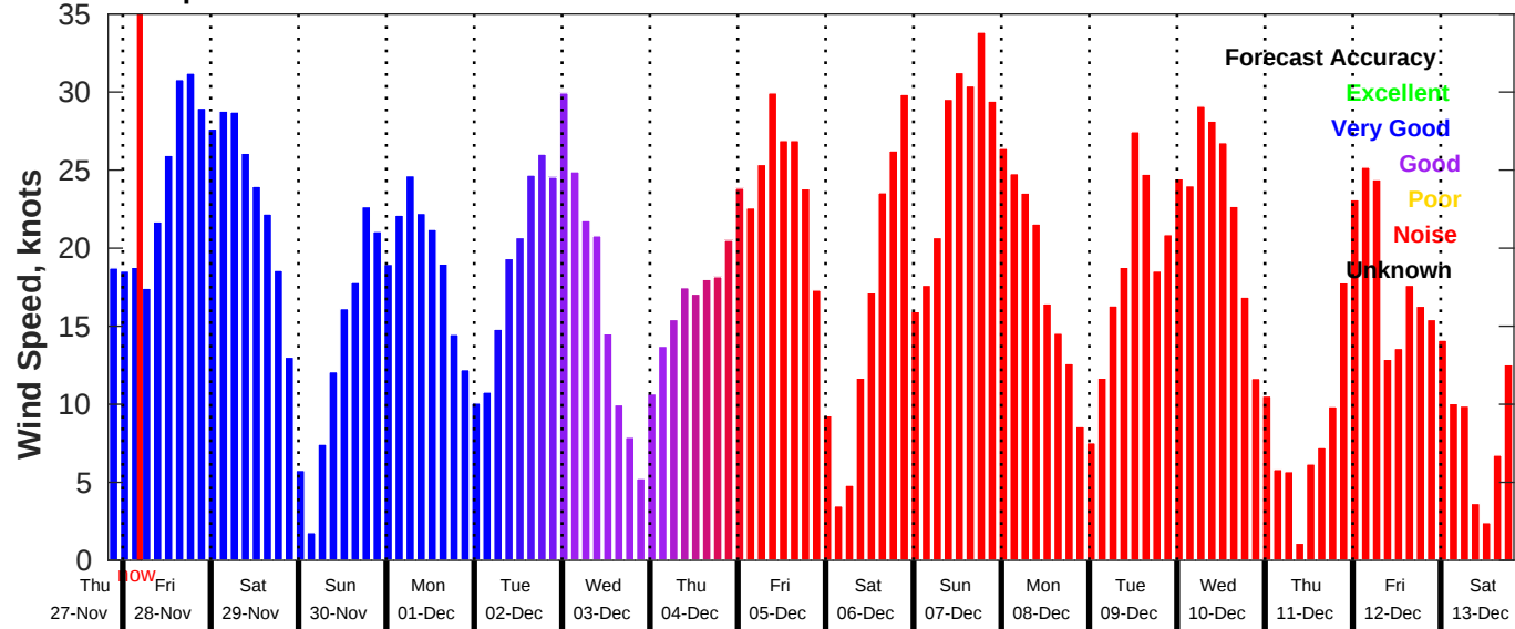
GFS Wind Speed Forecast for NDBC 44008 from 27-Nov-2025 20:00:00 to 13-Dec-2025 20:00:00
