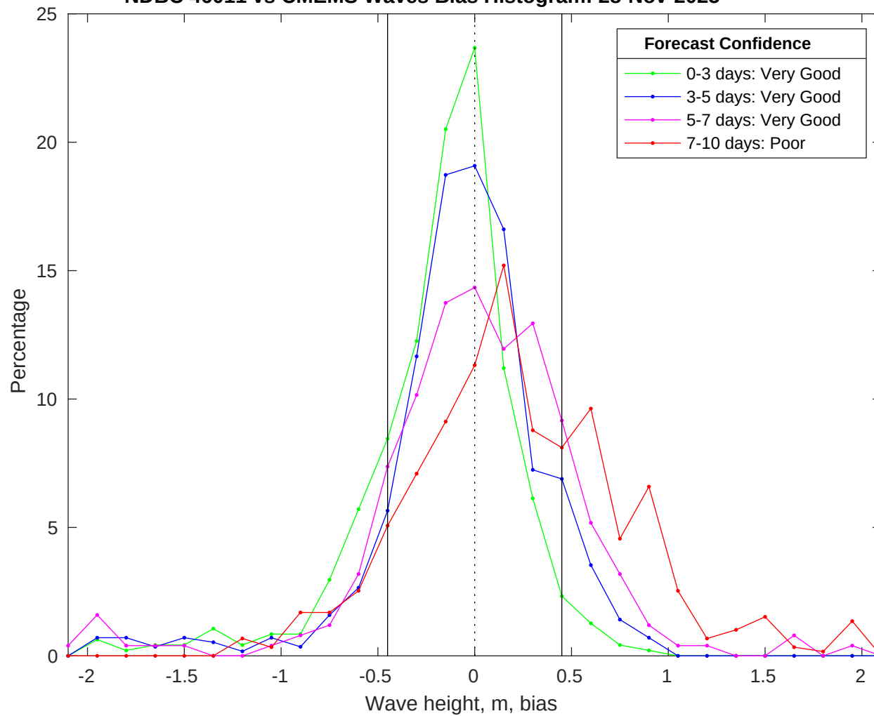
NDBC 46011 vs CMEMS Waves Bias Histogram: 28-Nov-2025
