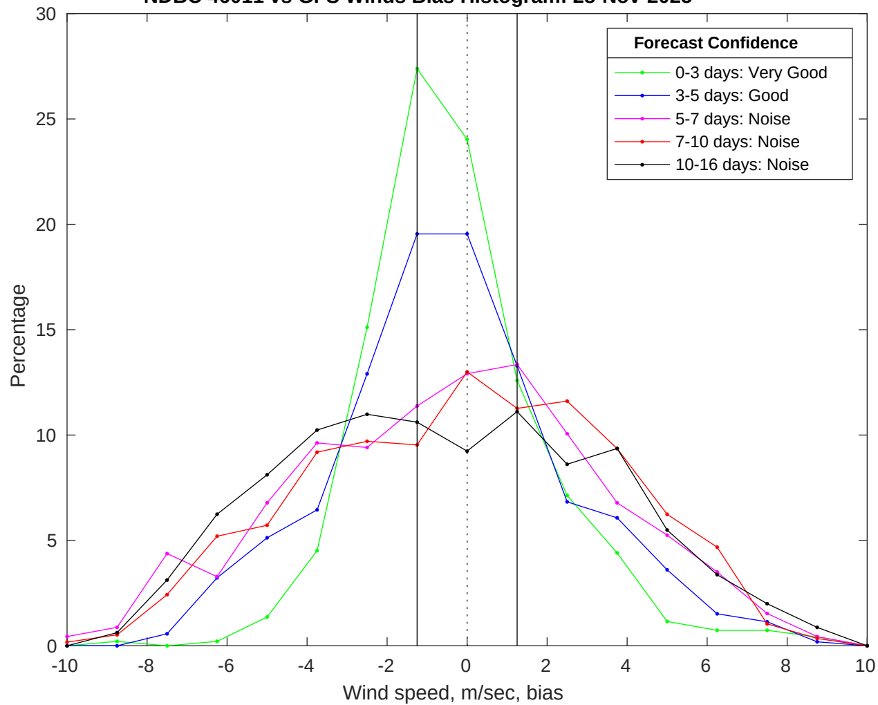
NDBC 46011 vs GFS Winds Bias Histogram: 28-Nov-2025
