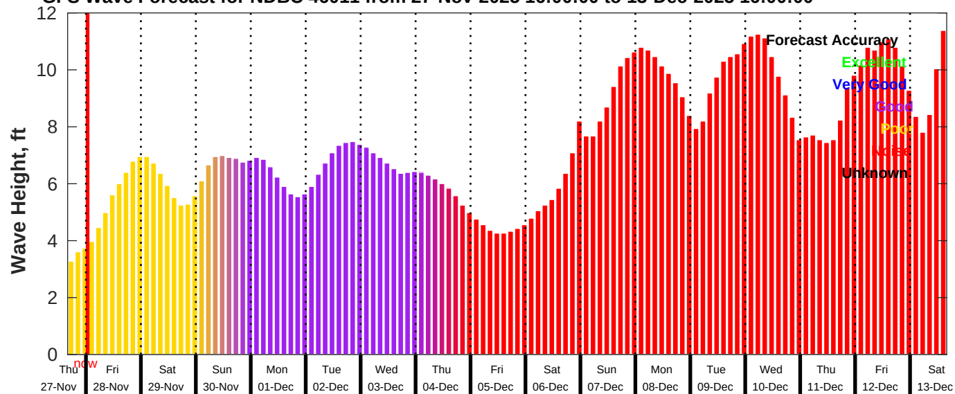
GFS Wave Forecast for NDBC 46011 from 27-Nov-2025 16:00:00 to 13-Dec-2025 16:00:00
