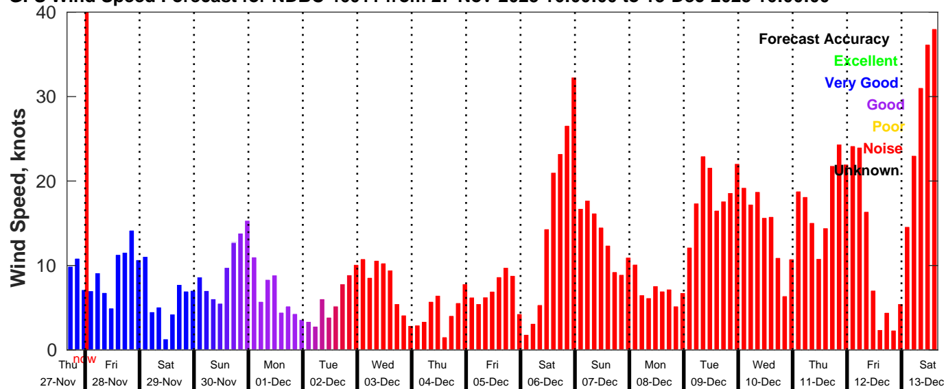
GFS Wind Speed Forecast for NDBC 46011 from 27-Nov-2025 16:00:00 to 13-Dec-2025 16:00:00
