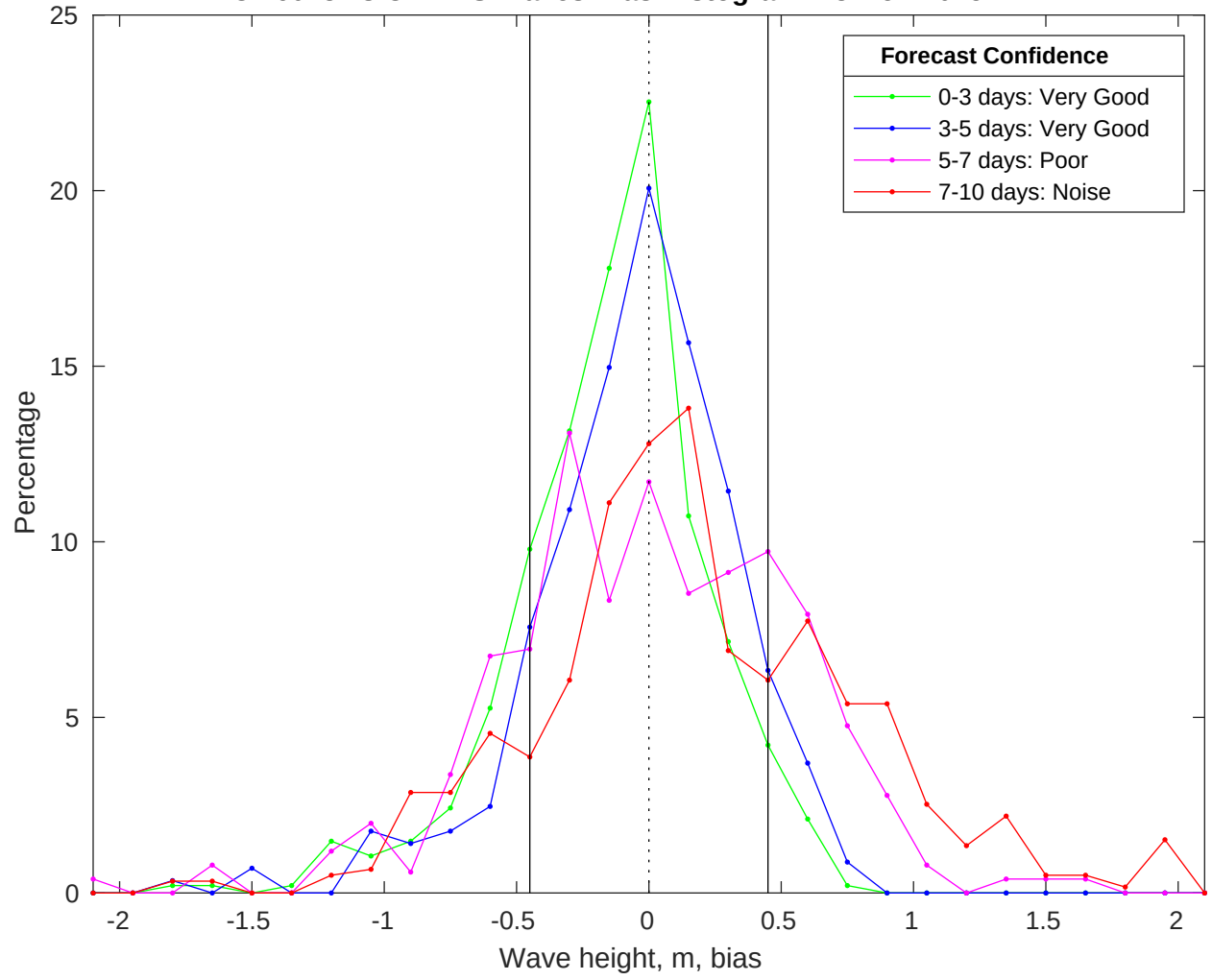
NDBC 46028 vs CMEMS Waves Bias Histogram: 28-Nov-2025
