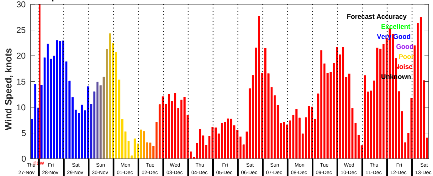
GFS Wind Speed Forecast for NDBC 46028 from 27-Nov-2025 16:00:00 to 13-Dec-2025 16:00:00
