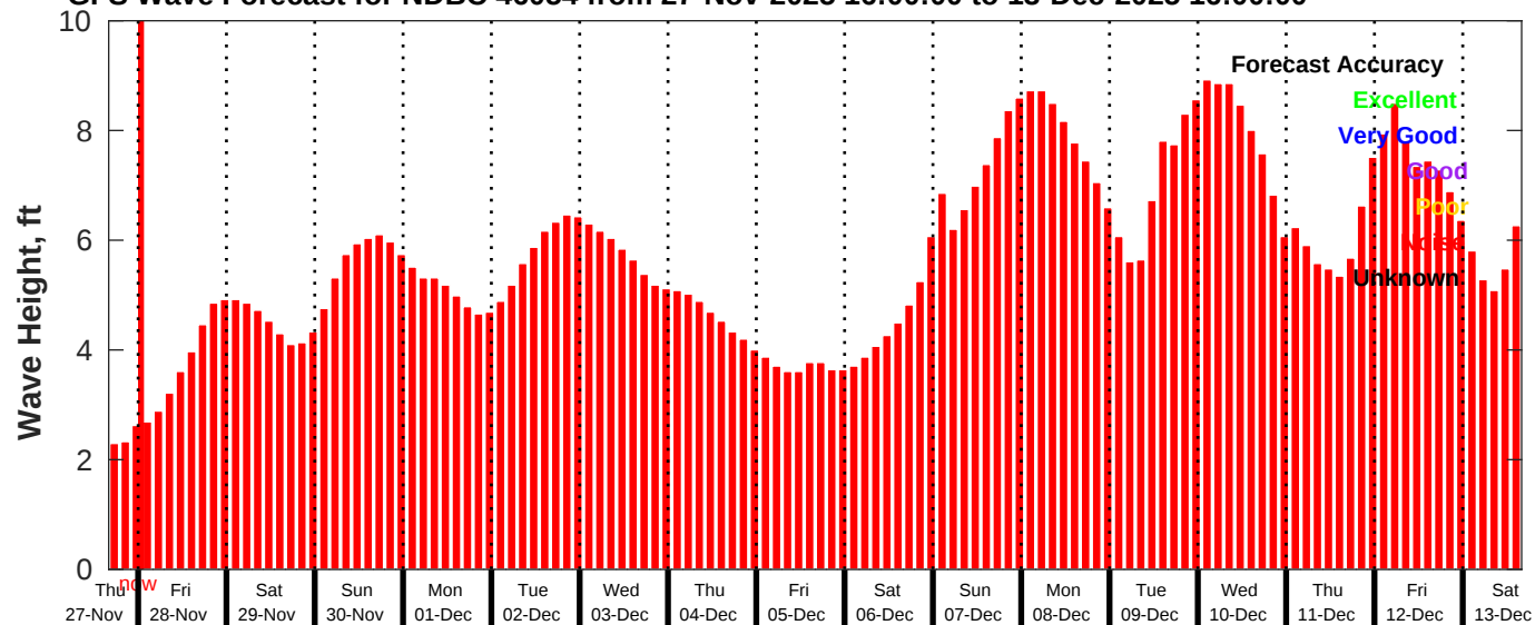
GFS Wave Forecast for NDBC 46054 from 27-Nov-2025 16:00:00 to 13-Dec-2025 16:00:00
