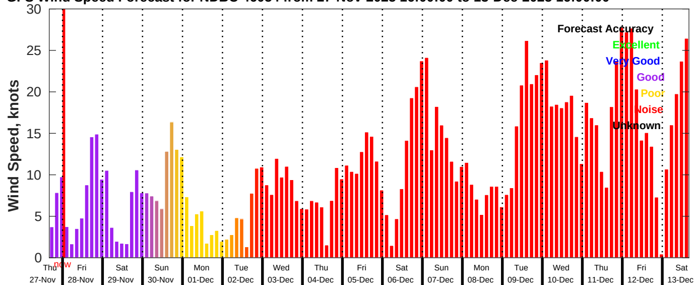
GFS Wind Speed Forecast for NDBC 46054 from 27-Nov-2025 16:00:00 to 13-Dec-2025 16:00:00
