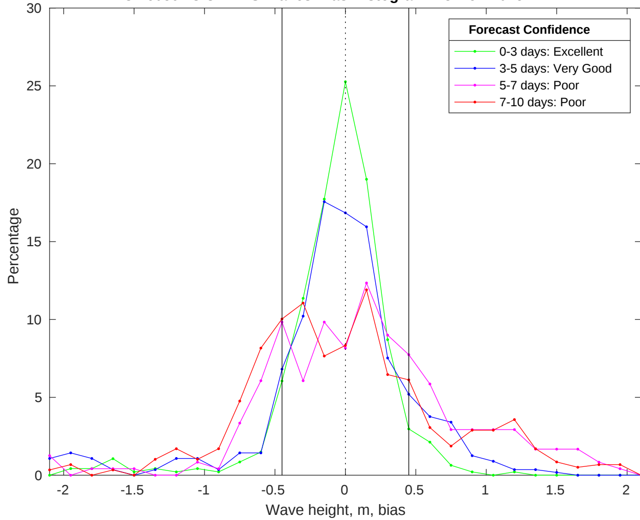
NDBC 46059 vs CMEMS Waves Bias Histogram: 28-Nov-2025
