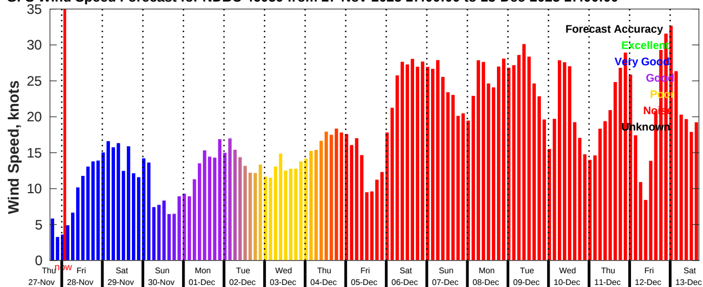
GFS Wind Speed Forecast for NDBC 46059 from 27-Nov-2025 17:00:00 to 13-Dec-2025 17:00:00
