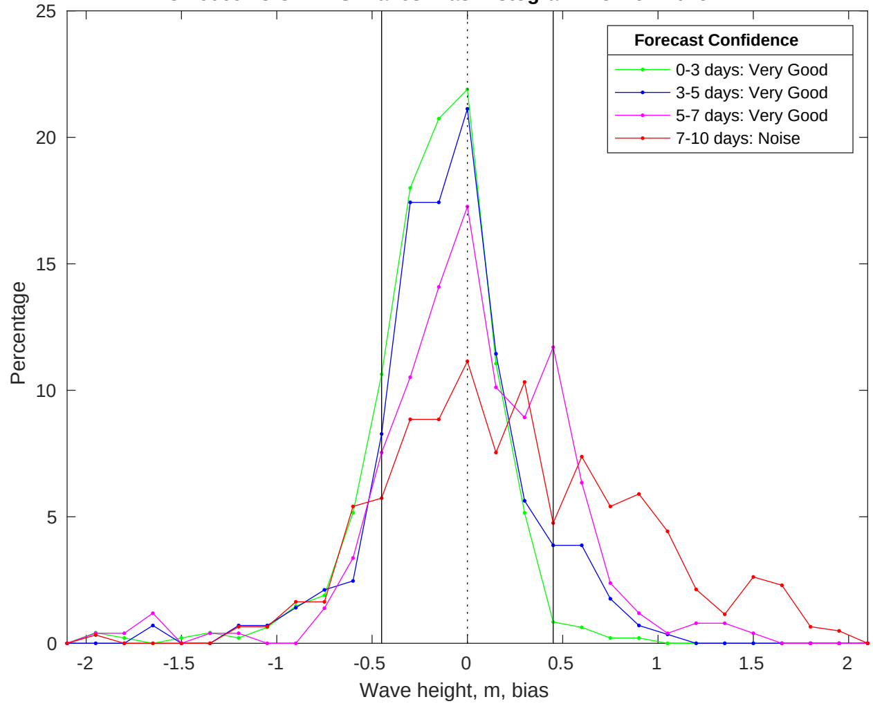
NDBC 46069 vs CMEMS Waves Bias Histogram: 28-Nov-2025
