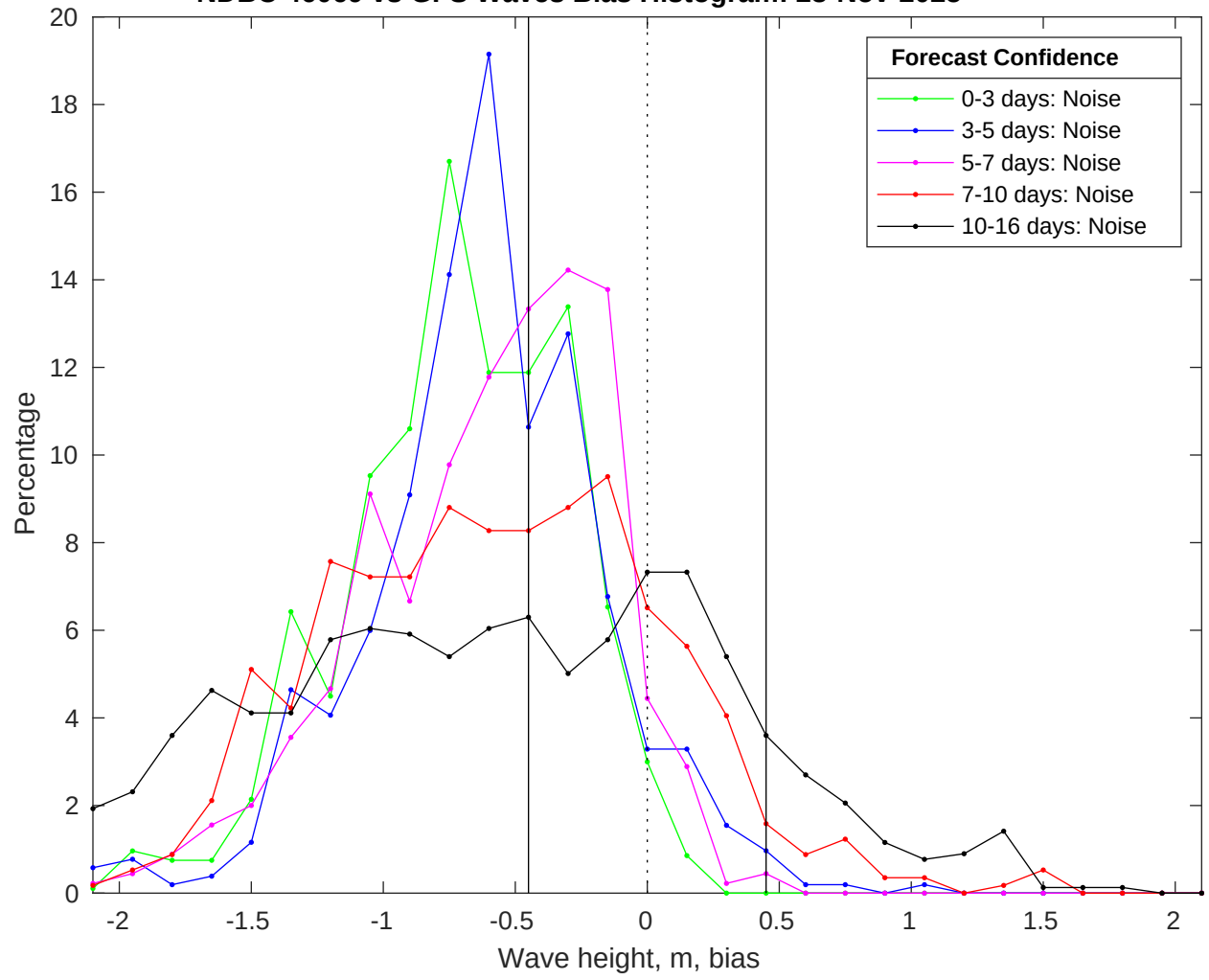
NDBC 46069 vs GFS Waves Bias Histogram: 28-Nov-2025
