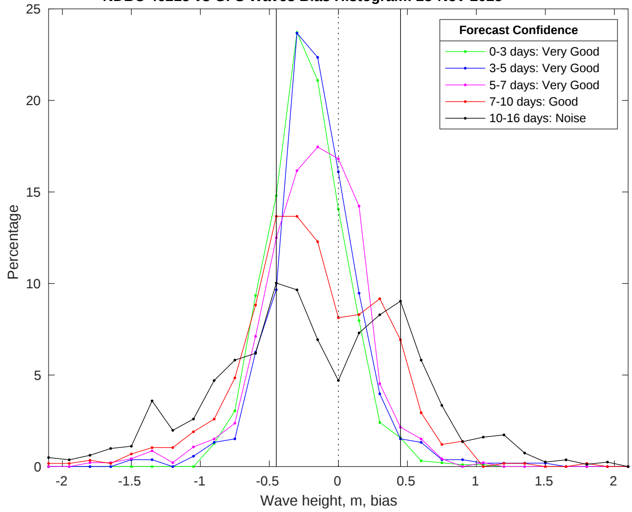
NDBC 46215 vs GFS Waves Bias Histogram: 28-Nov-2025
