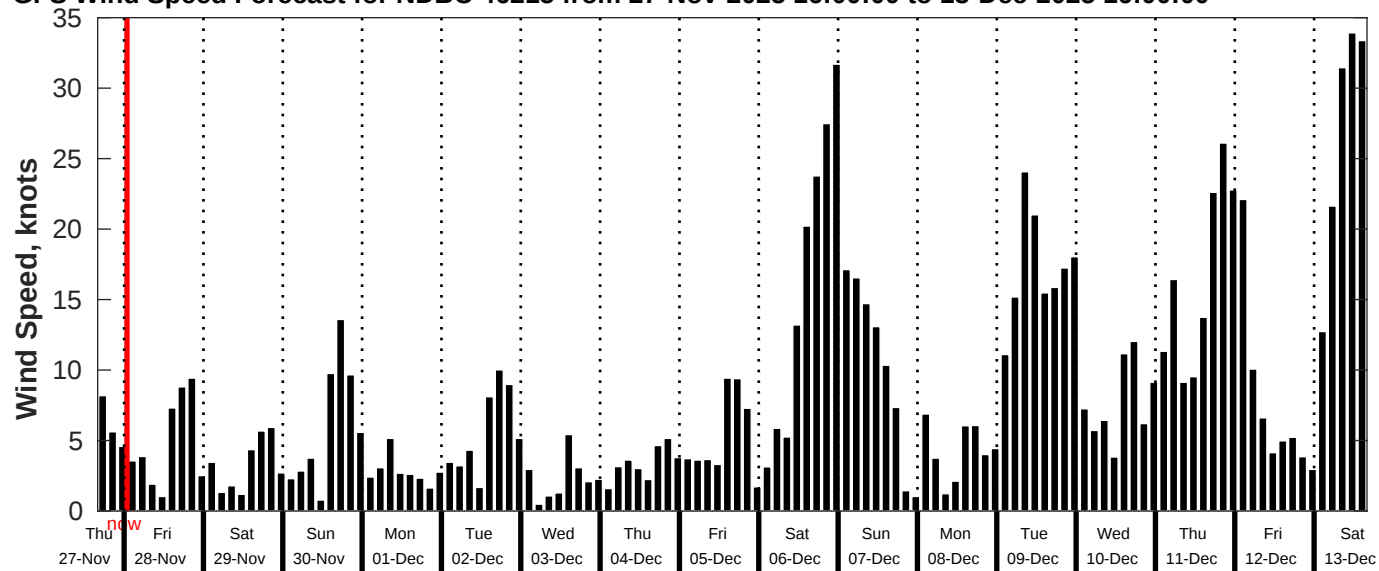
GFS Wind Speed Forecast for NDBC 46215 from 27-Nov-2025 16:00:00 to 13-Dec-2025 16:00:00
