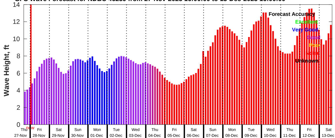
GFS Wave Forecast for NDBC 46259 from 27-Nov-2025 16:00:00 to 13-Dec-2025 16:00:00
