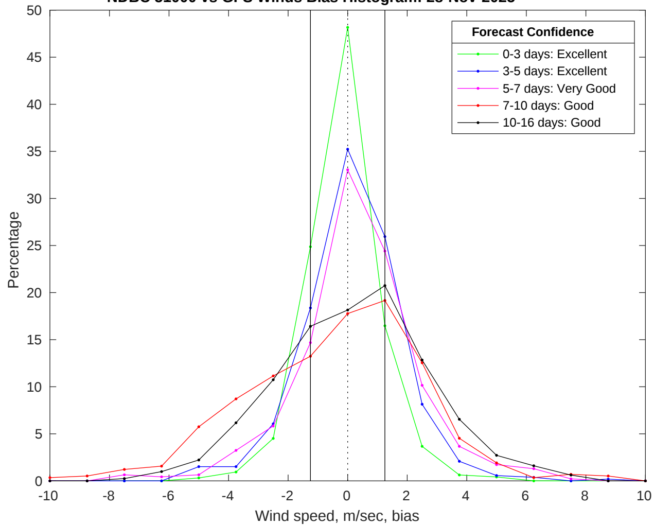
NDBC 51000 vs GFS Winds Bias Histogram: 28-Nov-2025
