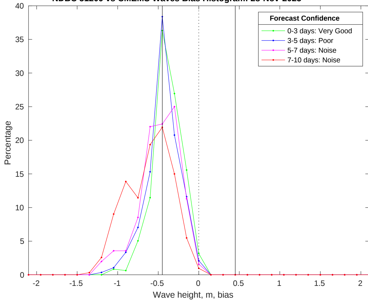
NDBC 51209 vs CMEMS Waves Bias Histogram: 28-Nov-2025
