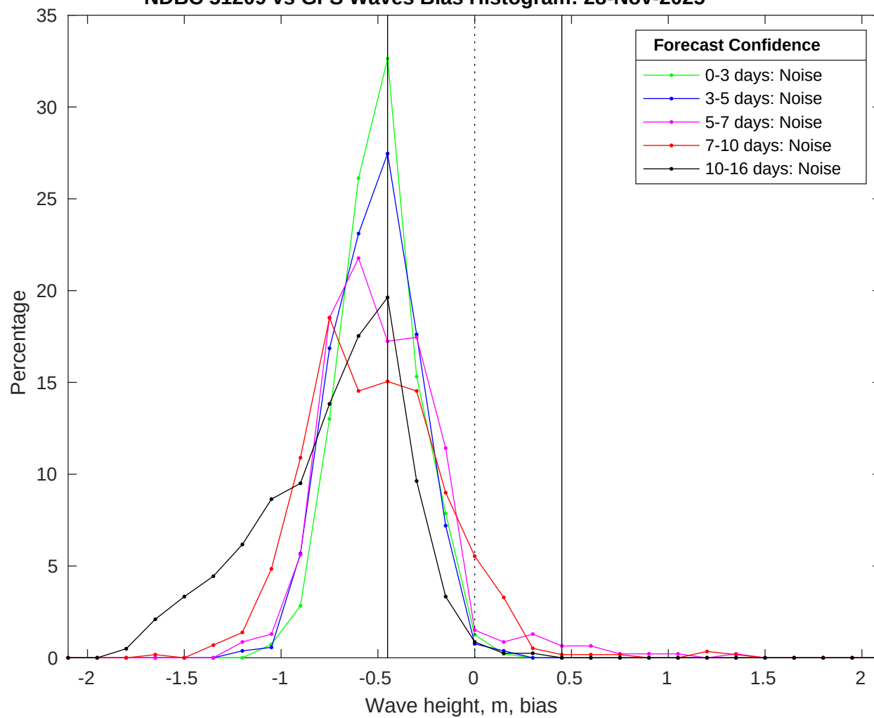
NDBC 51209 vs GFS Waves Bias Histogram: 28-Nov-2025
