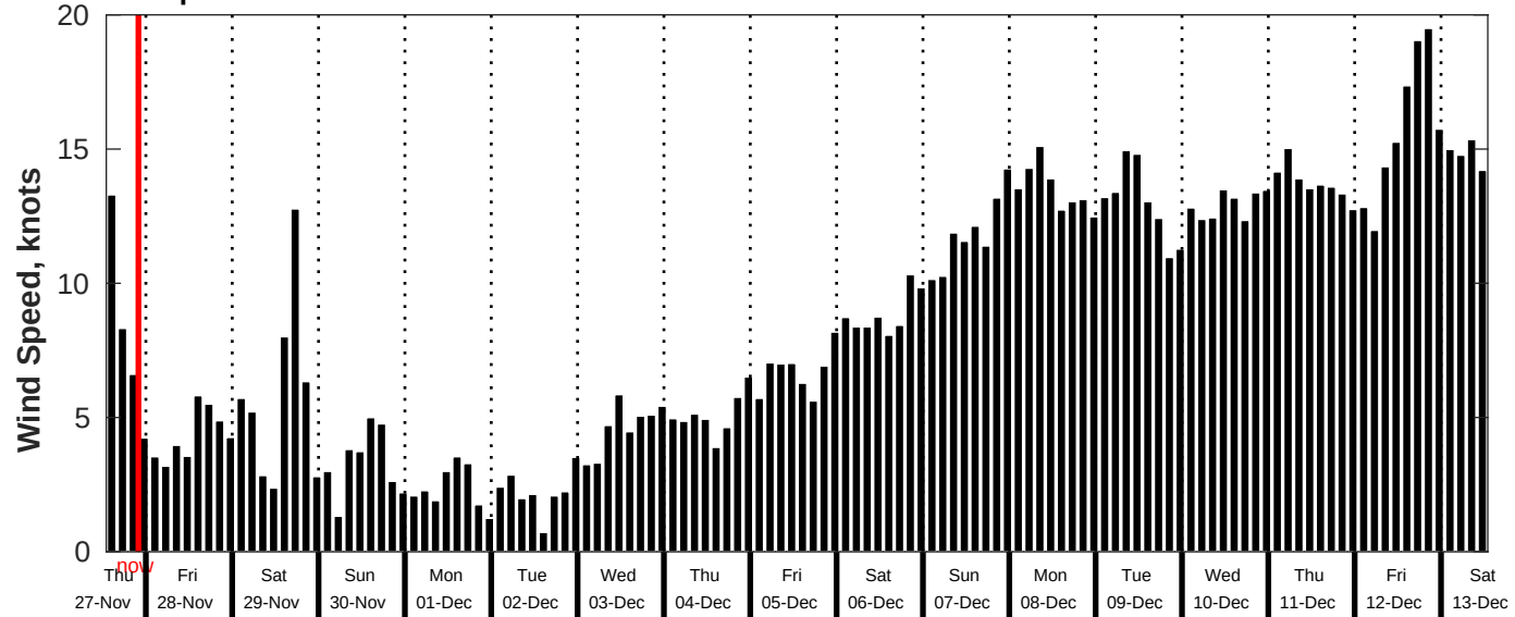
GFS Wind Speed Forecast for NDBC 51209 from 27-Nov-2025 13:00:00 to 13-Dec-2025 13:00:00
