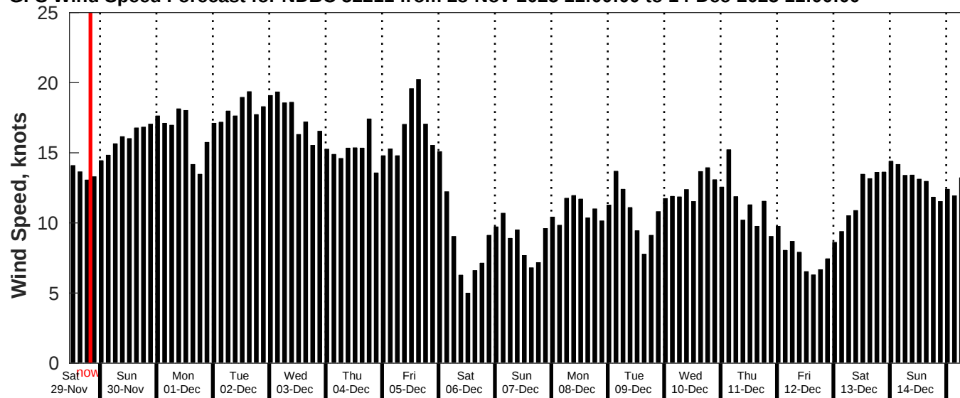
GFS Wind Speed Forecast for NDBC 52211 from 28-Nov-2025 11:00:00 to 14-Dec-2025 11:00:00
