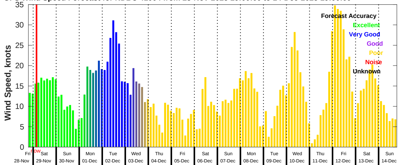
GFS Wind Speed Forecast for NDBC 41004 from 28-Nov-2025 19:00:00 to 14-Dec-2025 19:00:00
