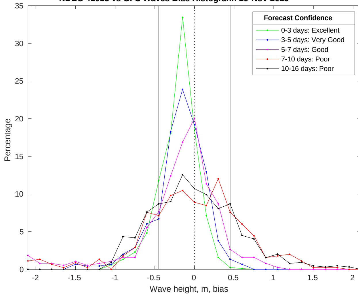
NDBC 41013 vs GFS Waves Bias Histogram: 29-Nov-2025
