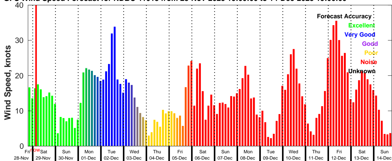
GFS Wind Speed Forecast for NDBC 41013 from 28-Nov-2025 19:00:00 to 14-Dec-2025 19:00:00
