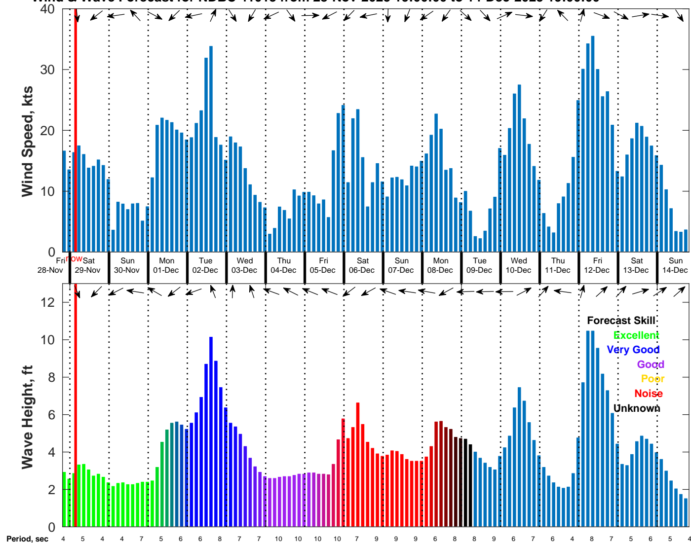
Wind & Wave Forecast for NDBC 41013 from 28-Nov-2025 19:00:00 to 14-Dec-2025 19:00:00
