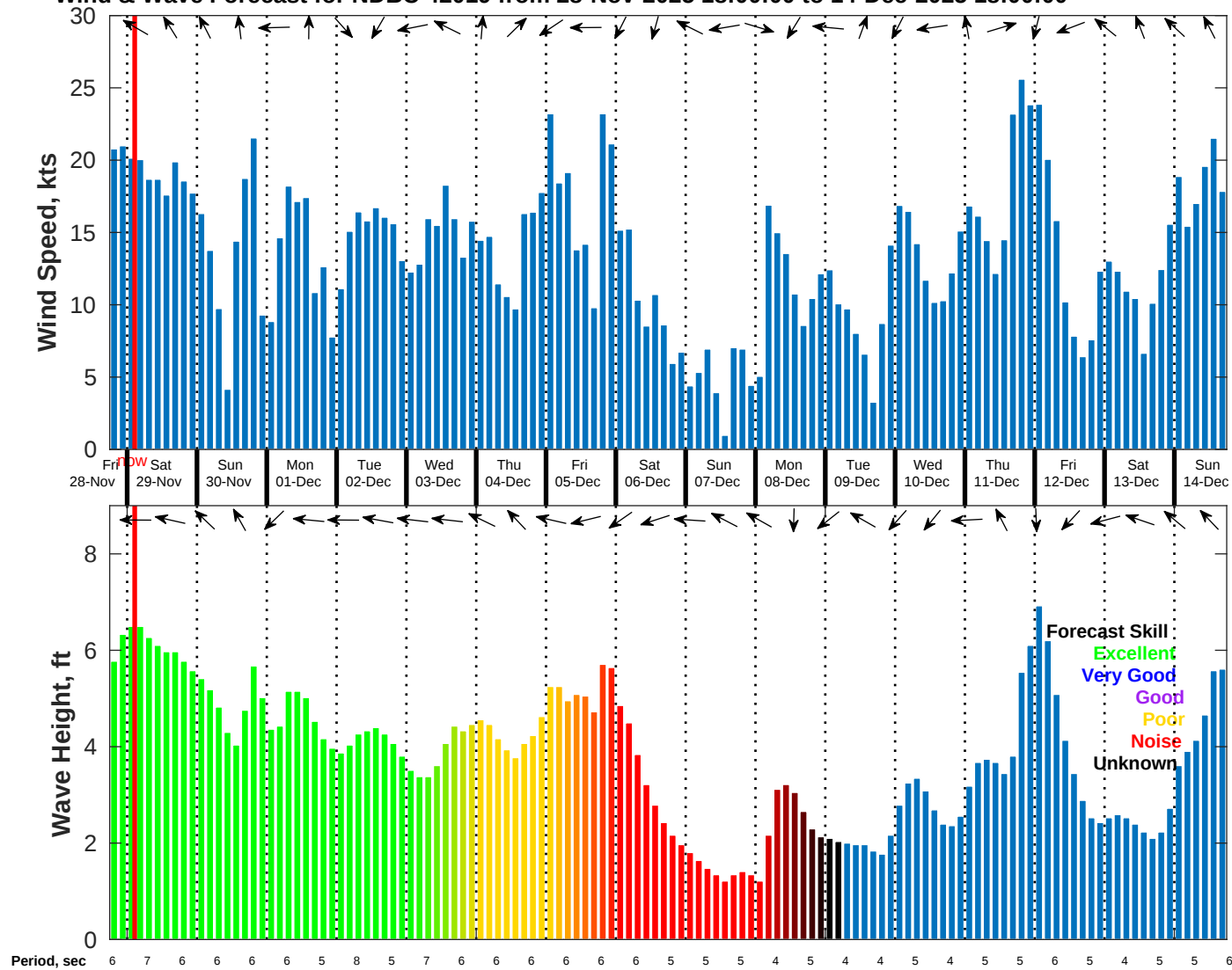
Wind & Wave Forecast for NDBC 42019 from 28-Nov-2025 18:00:00 to 14-Dec-2025 18:00:00
