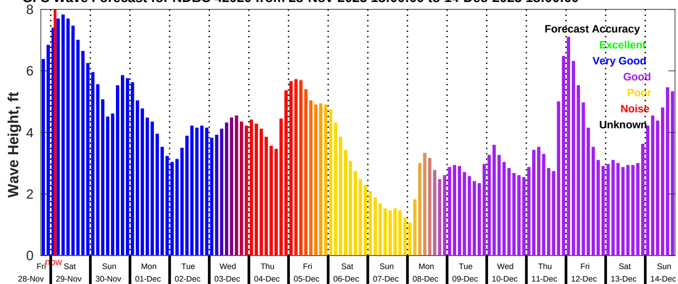
GFS Wave Forecast for NDBC 42020 from 28-Nov-2025 18:00:00 to 14-Dec-2025 18:00:00
