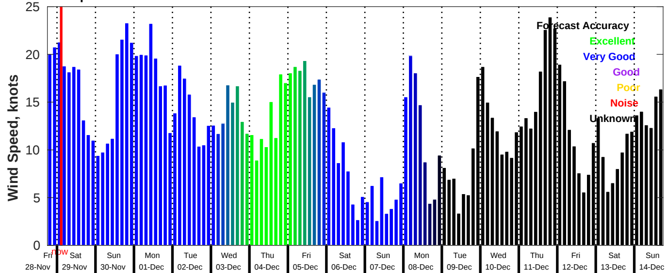
GFS Wind Speed Forecast for NDBC 42035 from 28-Nov-2025 18:00:00 to 14-Dec-2025 18:00:00
