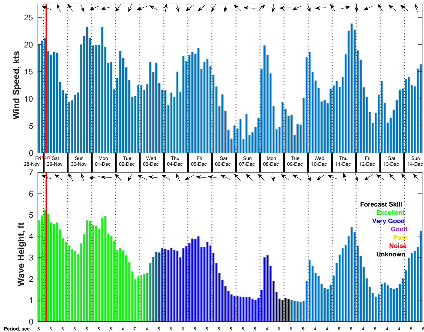
Wind & Wave Forecast for NDBC 42035 from 28-Nov-2025 18:00:00 to 14-Dec-2025 18:00:00
