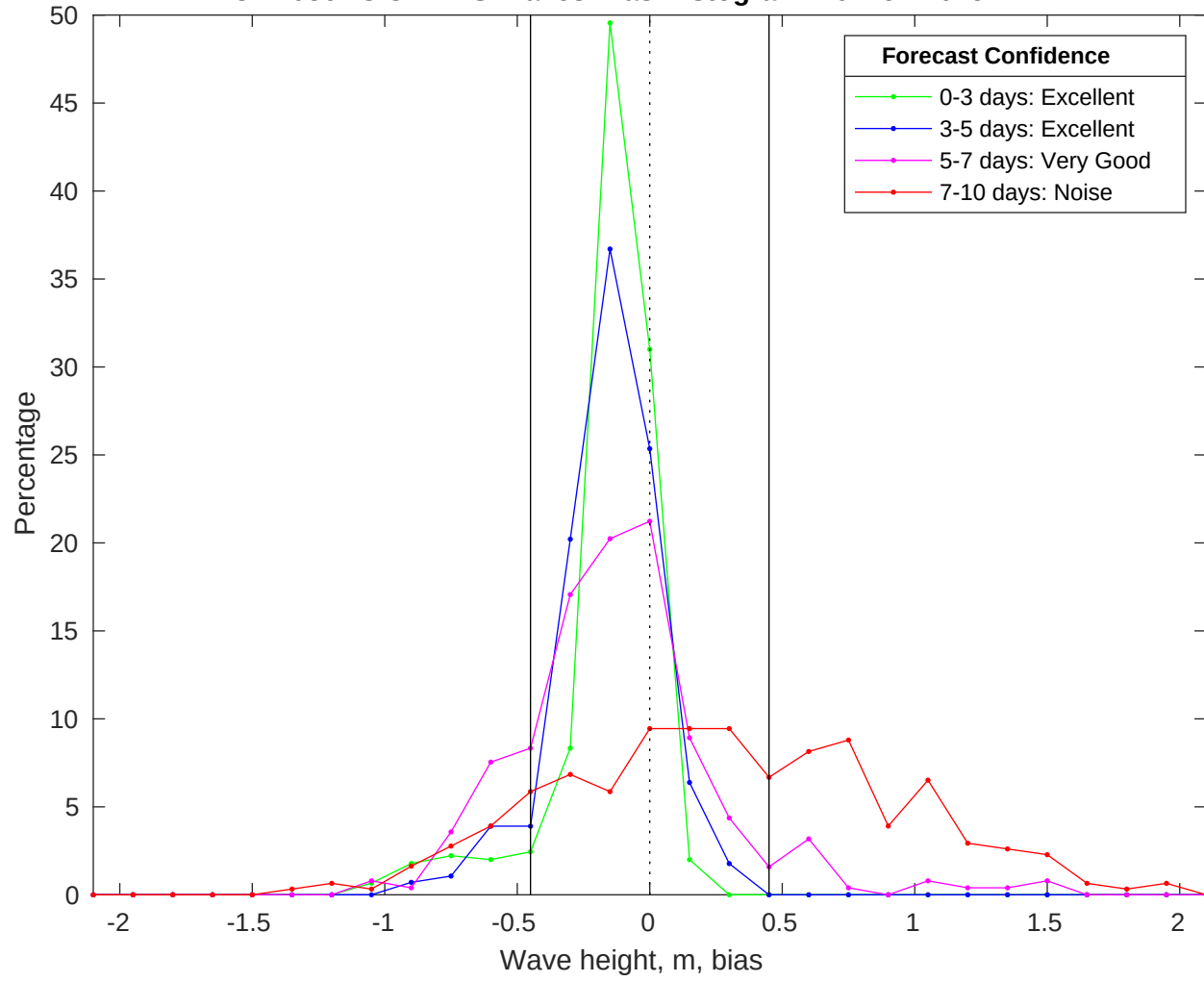
NDBC 42036 vs CMEMS Waves Bias Histogram: 29-Nov-2025
