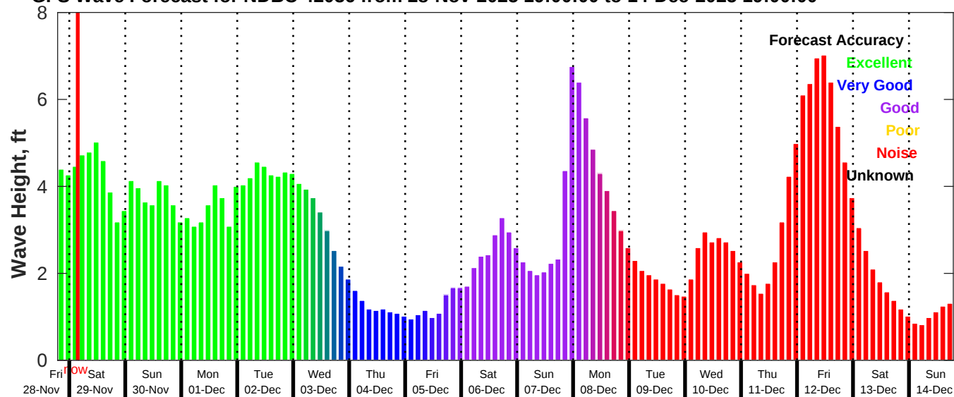
GFS Wave Forecast for NDBC 42036 from 28-Nov-2025 19:00:00 to 14-Dec-2025 19:00:00
