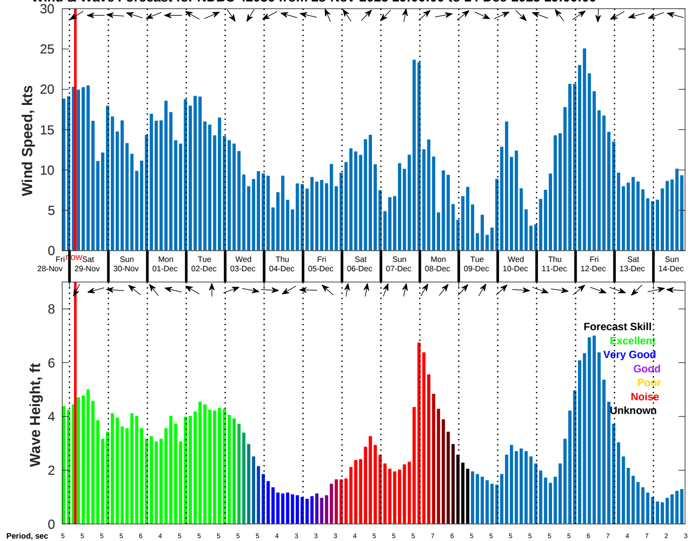
Wind & Wave Forecast for NDBC 42036 from 28-Nov-2025 19:00:00 to 14-Dec-2025 19:00:00
