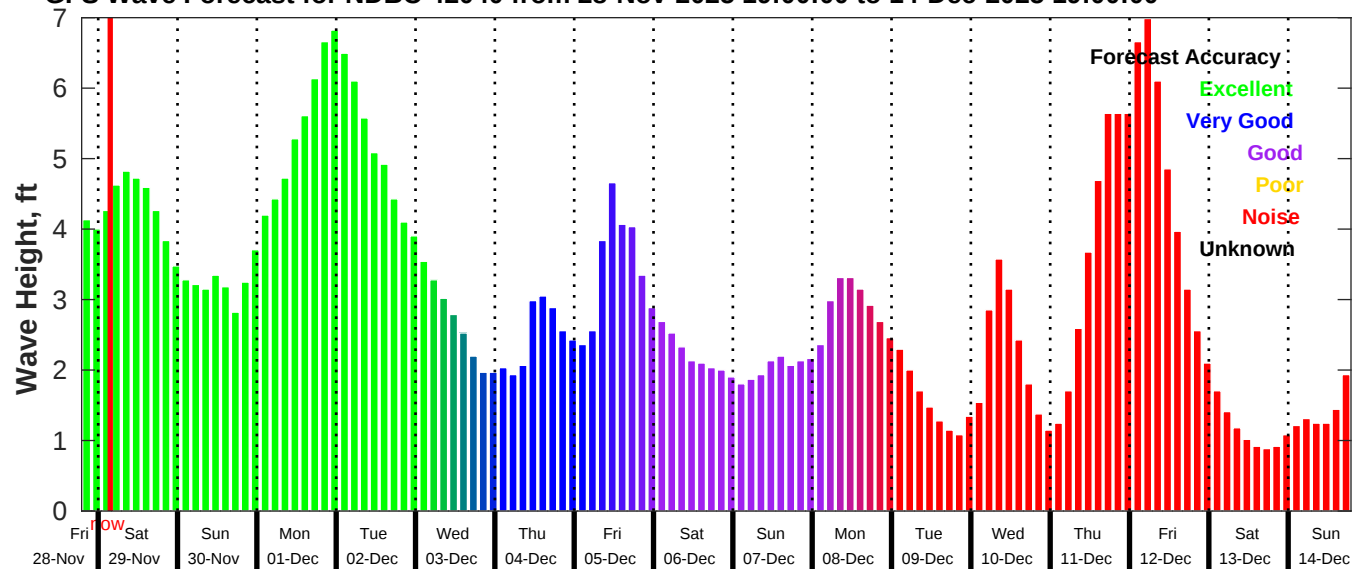
GFS Wave Forecast for NDBC 42040 from 28-Nov-2025 19:00:00 to 14-Dec-2025 19:00:00
