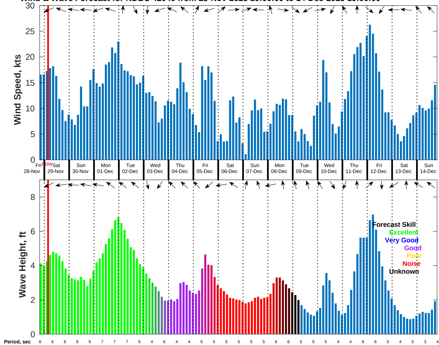
Wind & Wave Forecast for NDBC 42040 from 28-Nov-2025 19:00:00 to 14-Dec-2025 19:00:00
