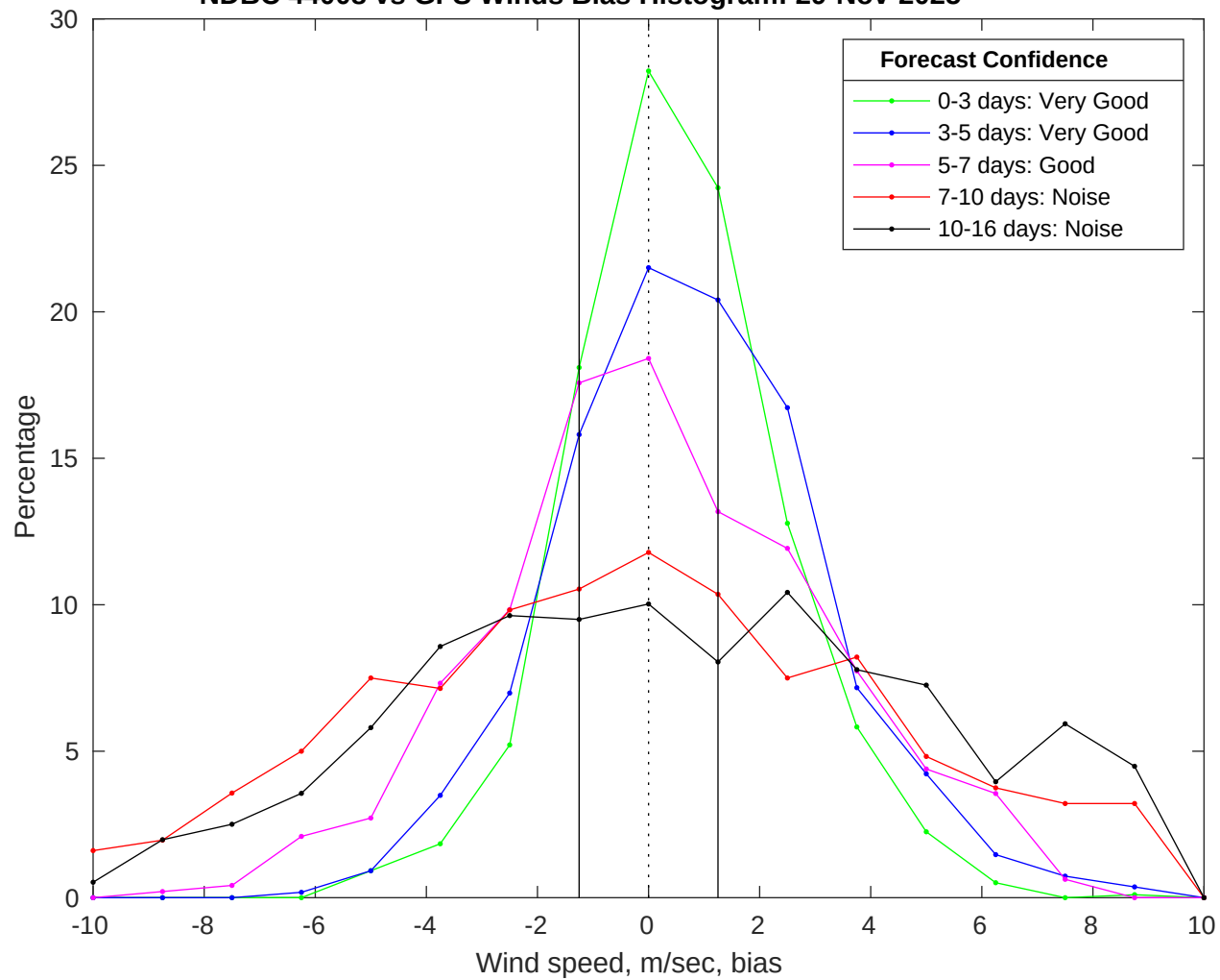
NDBC 44008 vs GFS Winds Bias Histogram: 29-Nov-2025
